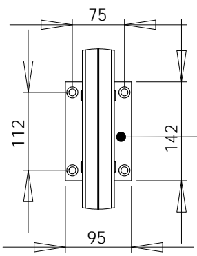
DETAIL B SCALE 2 : 15
