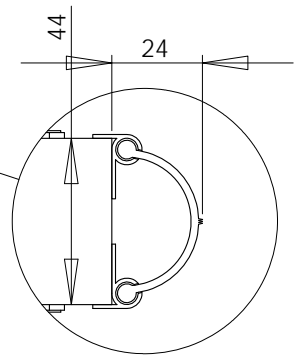
ANTI-FINGER TRAP SEAL DETAIL (DUAL EDGE) SCALE 1 : 2
